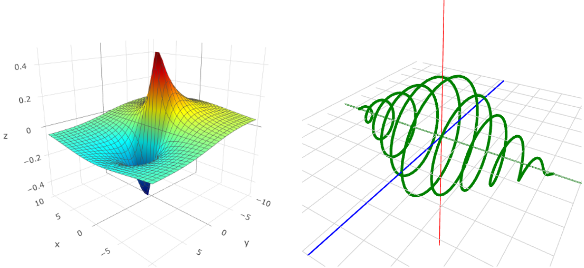
(a) BPST instanton: a finite-action, localized topological solution to the Yang–Mills equations, exhibiting geometric twist and winding [BPST75].
